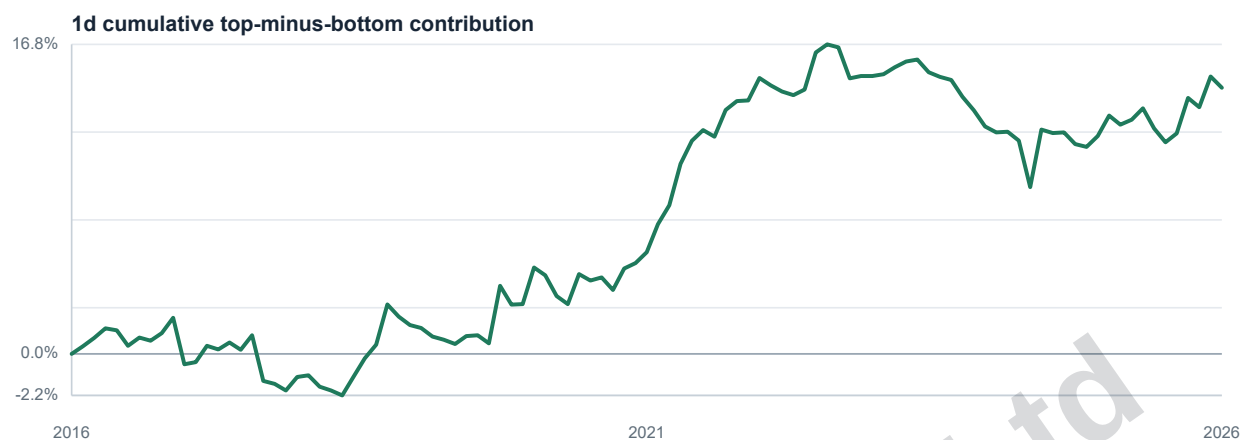
Figure 1. Cumulative 1d top-minus-bottom rank-spread contribution. Long-horizon forward observations can overlap, so the series should be read as a ranking diagnostic, not as a standalone portfolio NAV.
