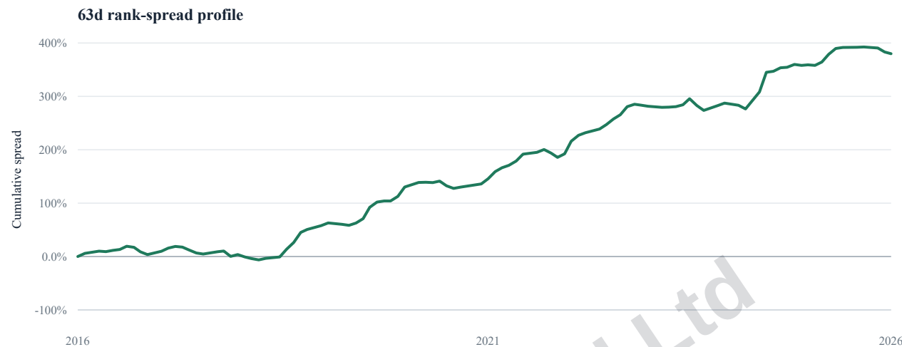
Figure 1. Cumulative 63d top-minus-bottom rank-spread contribution, normalised to zero at the first valid research observation. Long-horizon forward observations overlap, so the series should be read as a ranking diagnostic, not as a standalone return path.
